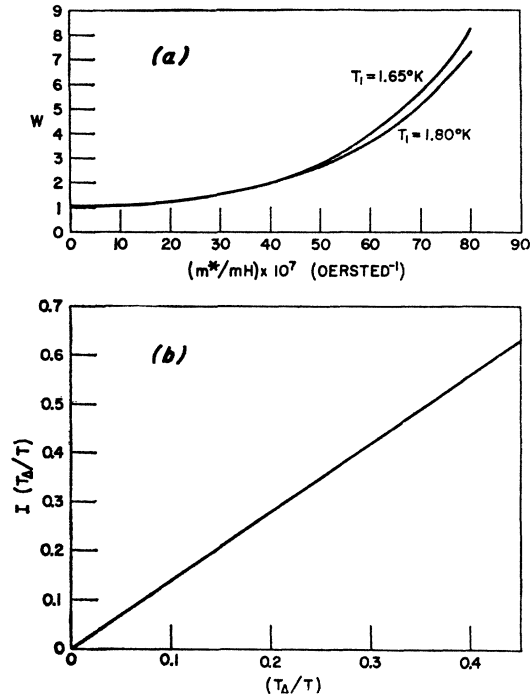
FIG. 6. (a) Calculated values of W as a function of (m^*/mH) ; (b) the function I(T_D/T) as a function of (T_D/T) .
