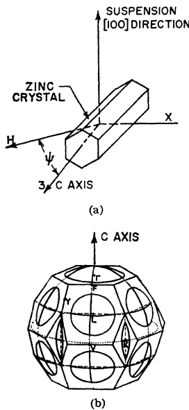
FIG. 1. (a) The orientation of the zinc crystals. (b) The Fermi surface of zinc [after E. Fawcett, J. Phys. Chem. Solids 18 , 320 (1961)]. The surfaces marked K are associated with the long-period de Haas-van Alphen effect.
