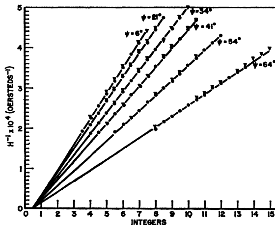
FIG. 4. The values of H^{-1} at extreme values of the torque as a function of half-integers for the 0.008 wt. % zinc manganese alloy. \bullet indicate data obtained at 4.2^\circ\text{K} ; \blacktriangledown indicate data obtained at 1.7^\circ\text{K} .
