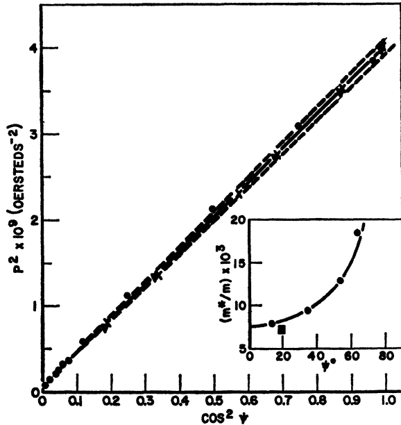
FIG. 5. P^2 as a function of \cos^2\psi . \nabla indicate data for pure zinc; \bullet indicate data for pure zinc obtained by Verkin and Dmitrenko; \times indicate data for the 0.008 wt. % zinc manganese alloy; the dotted lines indicate the experimental error; the inset shows m^*/m as a function of orientation for pure zinc; \blacksquare indicates the value obtained by Dhillon and Shoenberg.
