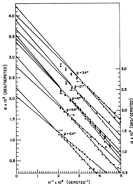
FIG. 8. Field dependence of the amplitude of the oscillations for the 0.008 wt. % zinc manganese alloy. ● indicates data obtained at 4.2°K; ■ indicates data obtained at 2.6°K; ▼ indicates data obtained at 1.7°K.
