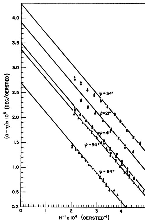
FIG. 9. Field dependence of the amplitude of the oscillations in the 0.008 wt. % zinc manganese alloy allowing for the postulated energy-dependent relaxation time. ● indicates data obtained at 4.2°K; ■ indicates data obtained at 2.6°K; ▲ indicates data obtained at 1.7°K.
