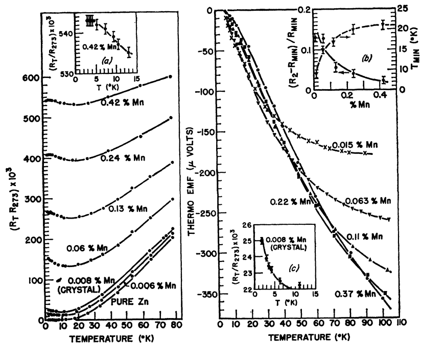
FIG. 2. The electrical resistance and thermo-emf as a function of temperature. Insets a , b , and c are referred to in the text.
