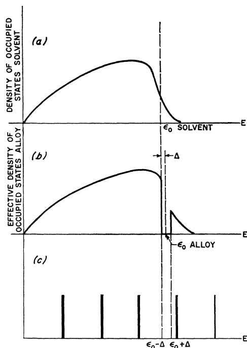
FIG. 10. (a) The density of populated states as a function of energy for the pure metal. (b) The effective density of states as a function of energy for an alloy having the postulated energy dependent relaxation time. (c) A schematic representation of the magnetic energy levels which give rise to the de Haas-van Alphen effect. Populated levels are indicated by heavy lines.
