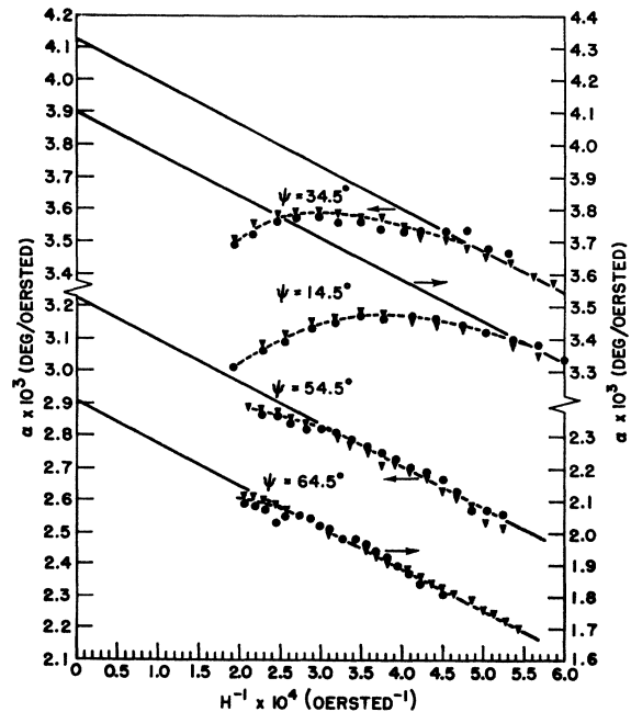
FIG. 7. Field dependence of the amplitude of the oscillations for pure zinc. ● indicates data obtained at 4.2 ^{\circ} K; ▼ indicates data obtained at 1.7 ^{\circ} K.
