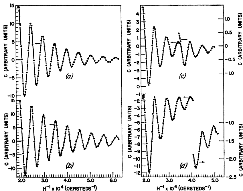
FIG. 3. The experimental results of the de Haas-van Alphen effect measurements. (a) pure zinc T=4.2^\circ\text{K} , \psi=34.5^\circ ; (b) pure zinc T=1.75^\circ\text{K} , \psi=34.5^\circ ; (c) 0.008 wt. % zinc manganese alloy T=4.2^\circ\text{K} , \psi=34.0^\circ ; (d) 0.008 wt. % zinc manganese alloy T=1.65^\circ\text{K} , \psi=34.0^\circ . The vertical asymmetry of the oscillations is probably due to the influence of the anisotropic crystalline environment of the manganese ions and is presently undergoing further investigation.
